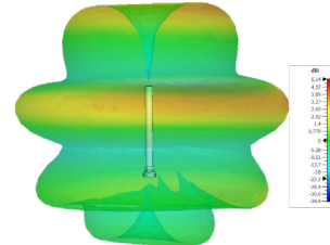
3D Plot Bottom Element (2170 MHz)
