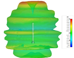
3D Plot Bottom Element (3600 MHz)
