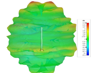
3D Plot Bottom Element (5400 MHz)
