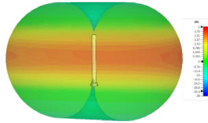
3D Plot Bottom Element (700 MHz)
