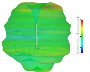
3D Plot Top Element (3600 MHz)
