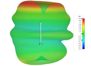
3D Plot Bottom Element (3600 MHz)
