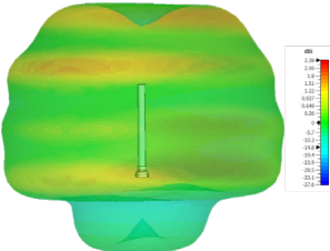
3D Plot Top Element (2170 MHz)
