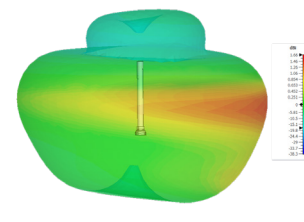
3D Plot Bottom Element (1800 MHz)
