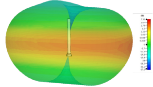
3D Plot Bottom Element (800 MHz)
