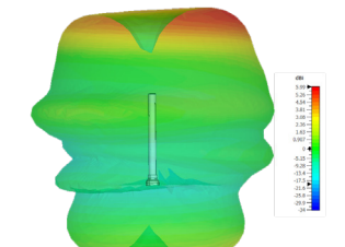
3D Plot Bottom Element (2600 MHz)
